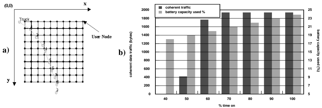
Figure 9: a) Sensor Scenario in Grid Sensor Network b) Coherent traffic data and the battery efficiency of various power cycle durations
